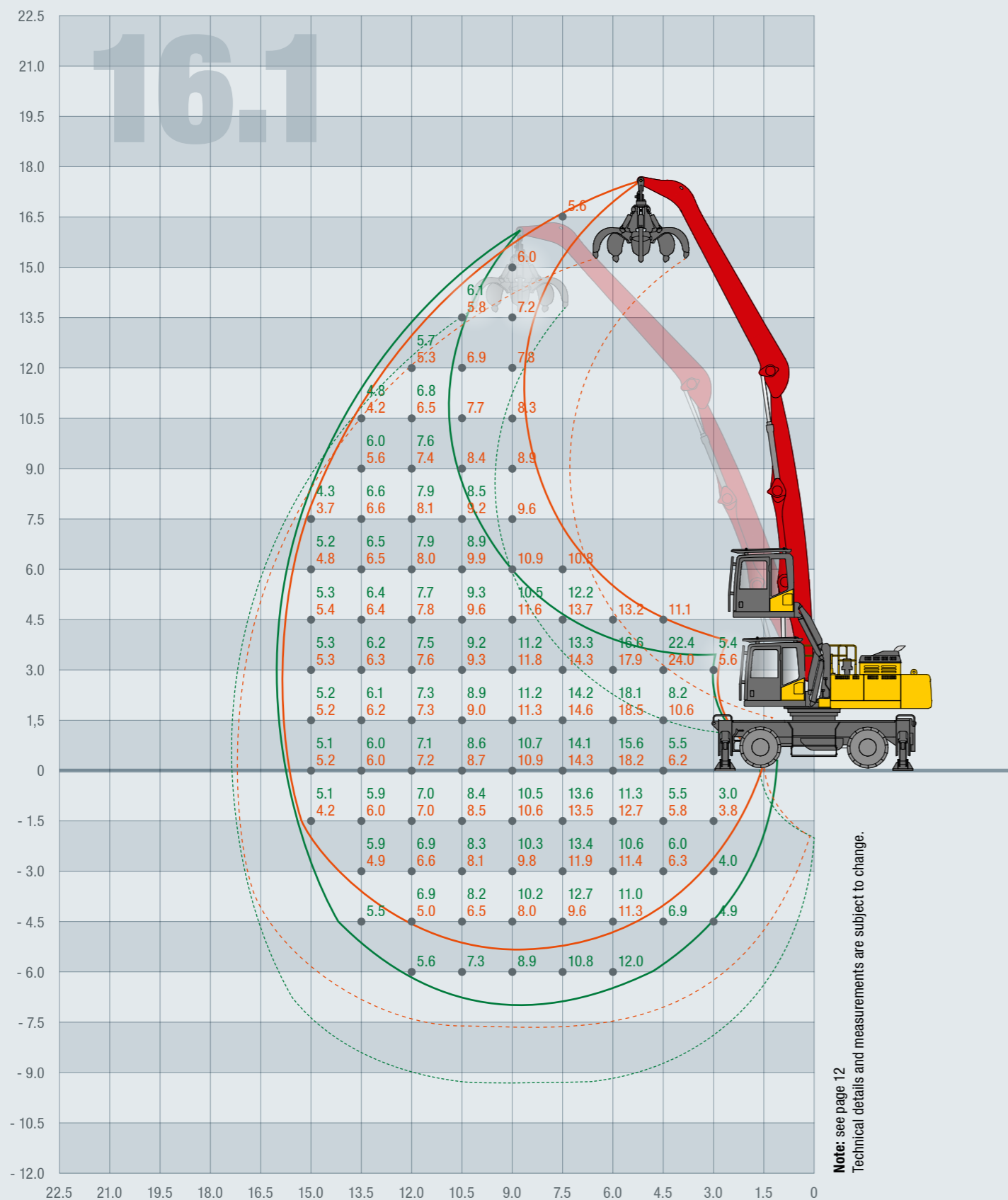
16.1 M LOWER FULL-FLOATING AXLE POSITION FOR BOOM INCREASED GRIPPING HEIGHT
