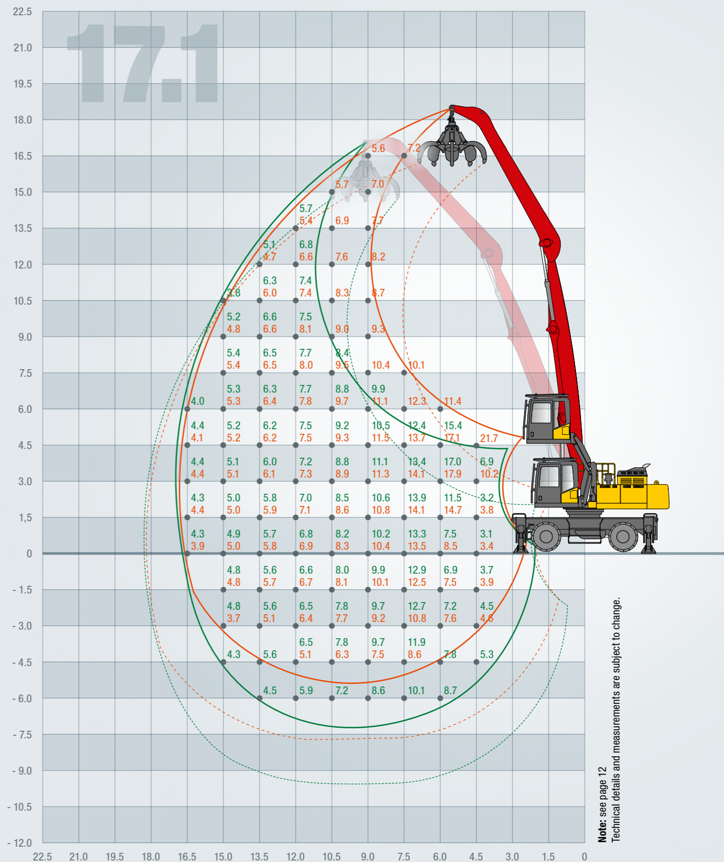
17.1 M LOWER FULL-FLOATING AXLE POSITION FOR BOOM INCREASED GRIPPING HEIGHT
