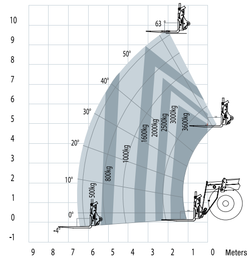
STH1133 – OUTRIGGERS UP
