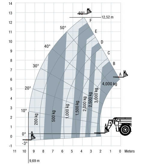
STH1840 – OUTRIGGERS UP
