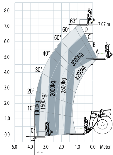
STH1133 – OUTRIGGERS DOWN
